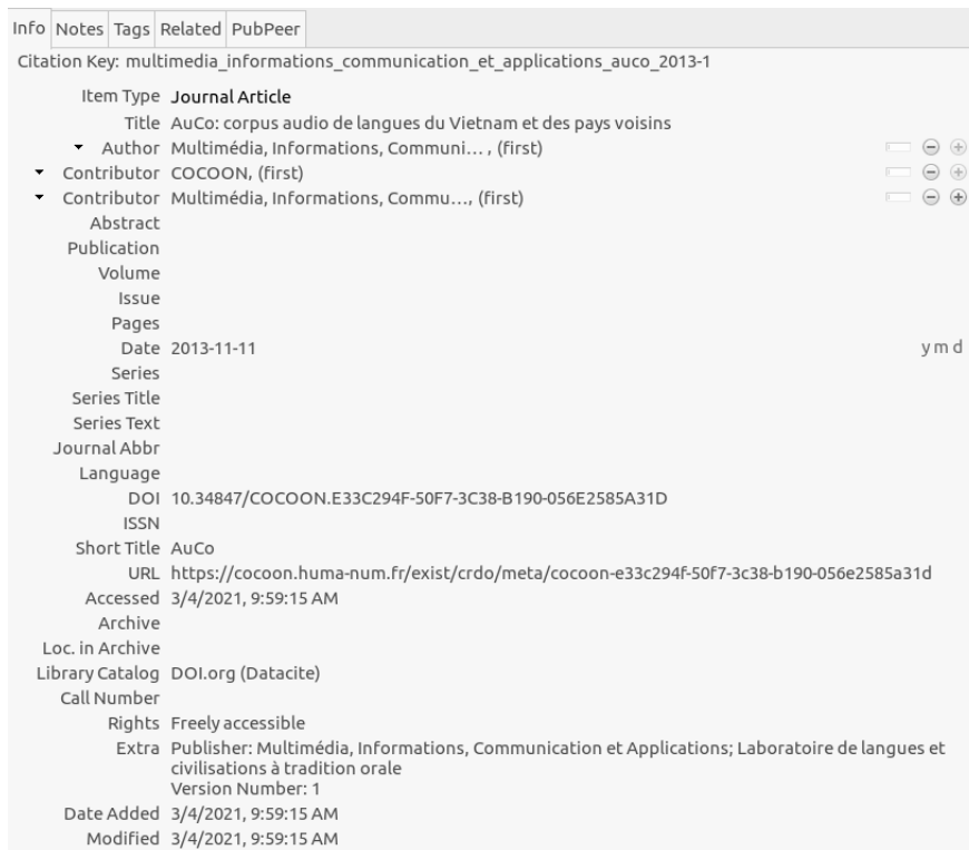
Figure 21. Zotero's interpretation of DataCite API supplied JSON for the Cocoon collection
