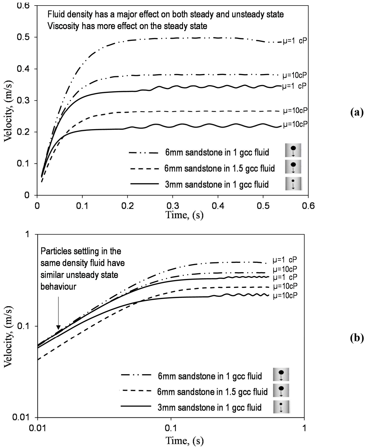
Figure 4.32 – Effect of particle size and fluid density and viscosity on the particle settling velocity using simulation: (a) Cartesian plot (b) log-log plot
