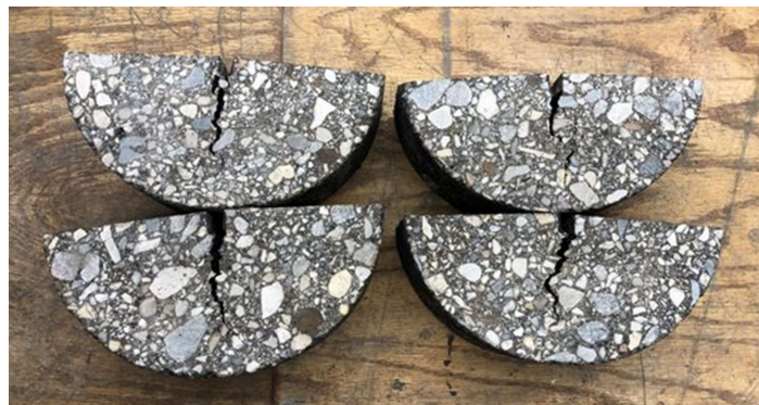
Figure 42. Typical sample after SCB test
