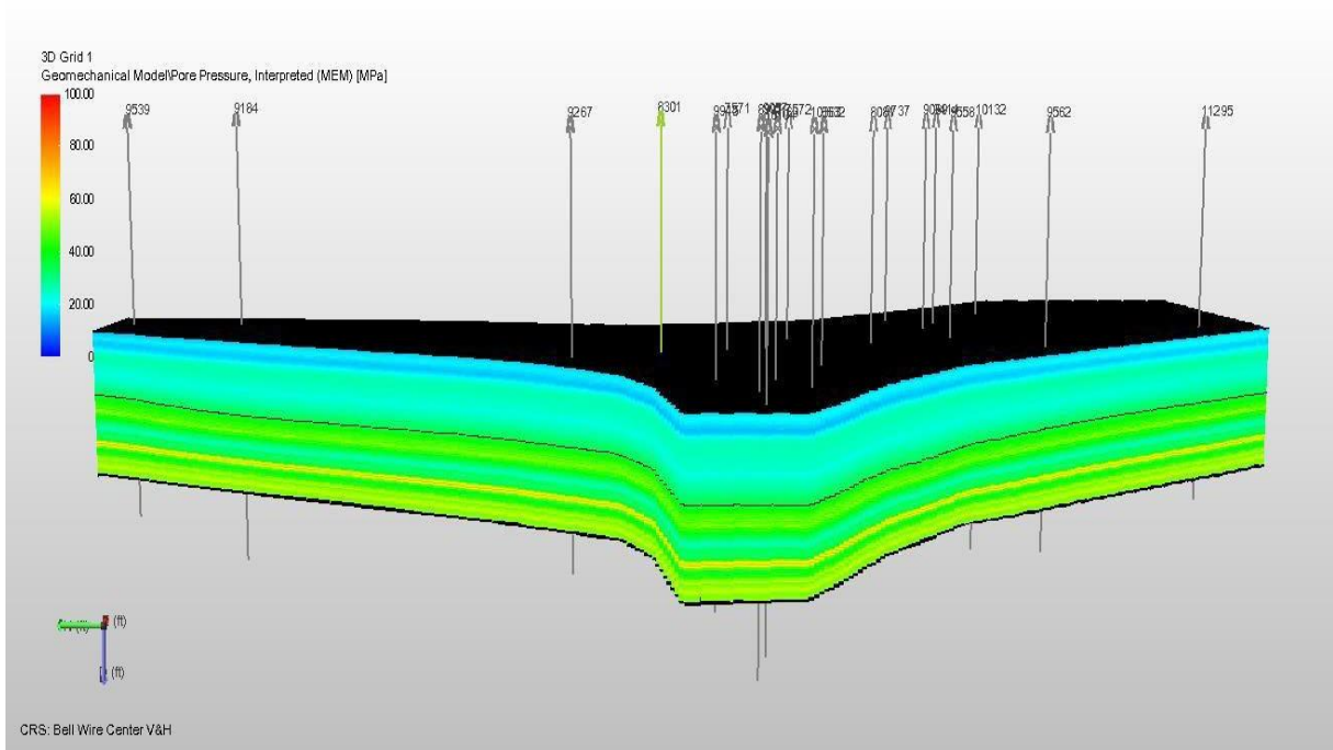
Fig (36). View of Blue Buttes grid populated with Interpreted Pore Pressure.
