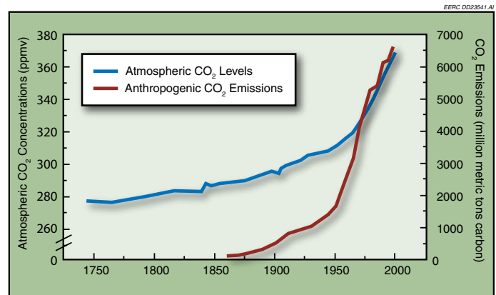
Since the beginning of large-scale industrialization about 150 years ago, the level of CO 2 in the atmosphere increased by about 25%. 1,5
