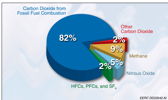
The diagram shows the contribution to global warming potential by gas type for the anthropogenic GHG emitted by the United States in 2001. Although a relatively weak GHG, CO 2 is emitted in such large quantities that it constitutes 84% of the global warming potential of the emissions.
