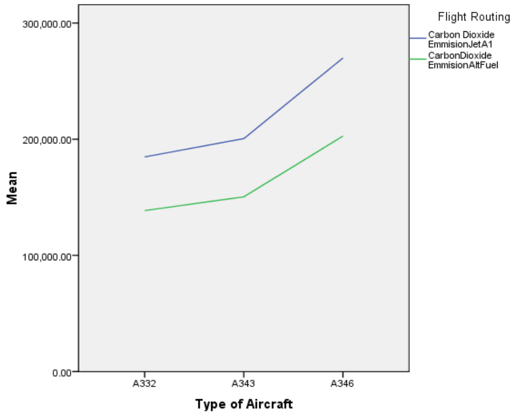
Figure 2. A plot of the mean CO 2 emission of SAA per fleet for flights to Europe using Jet A1 and Alternate Fuel blend.
