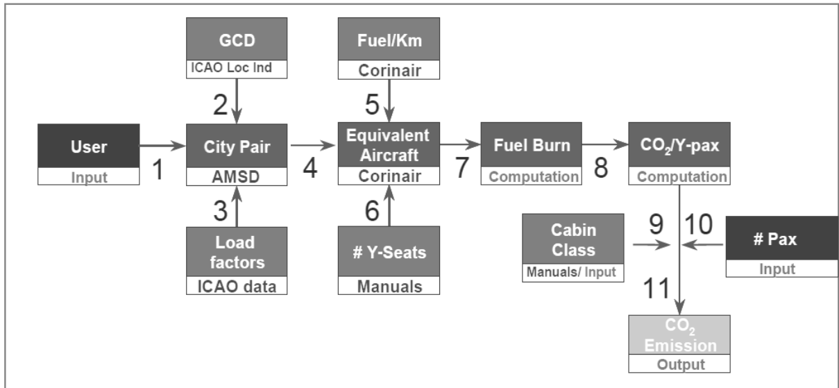
Figure 1. Flowchart of methodology used by ICAO /CORINAIR to determine the total emission of CO 2 produced by burning a ton of aviation fuel (ICAO, 2014)
