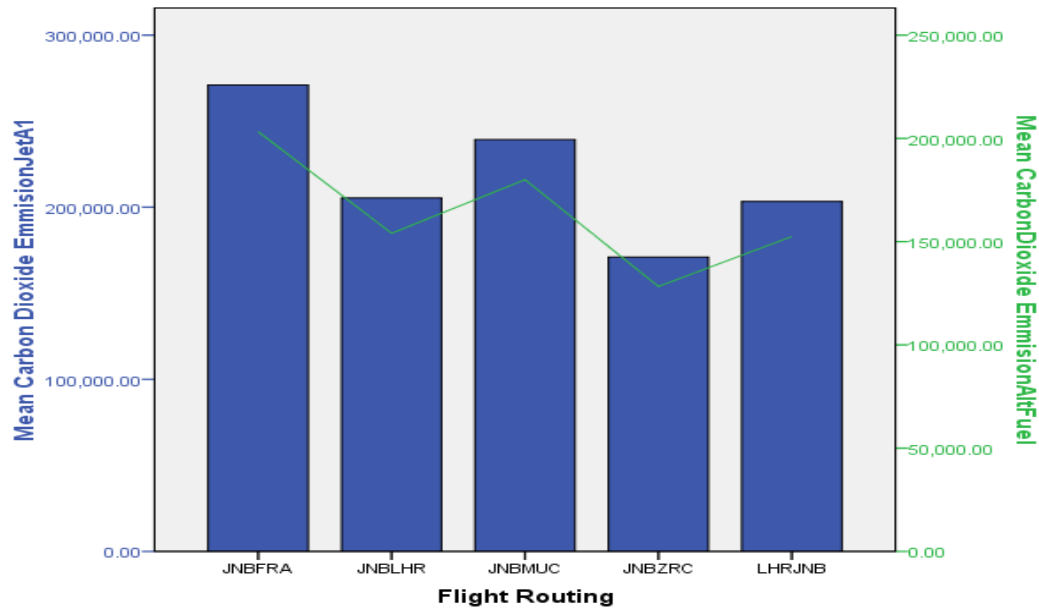
Figure 3. Mean Carbon Dioxide per SAA EU Flight Routings in Q1 FY14.
