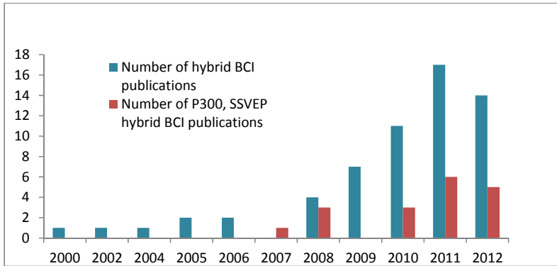
Figure 10. The increasing research trend in hybrid BCI area.
