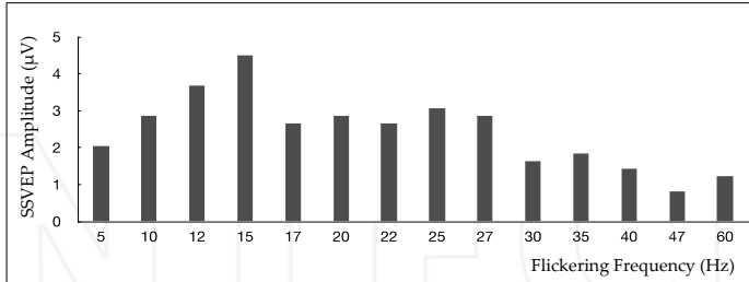
Figure 9. SSVEP amplitude with different flickering frequency [28].
