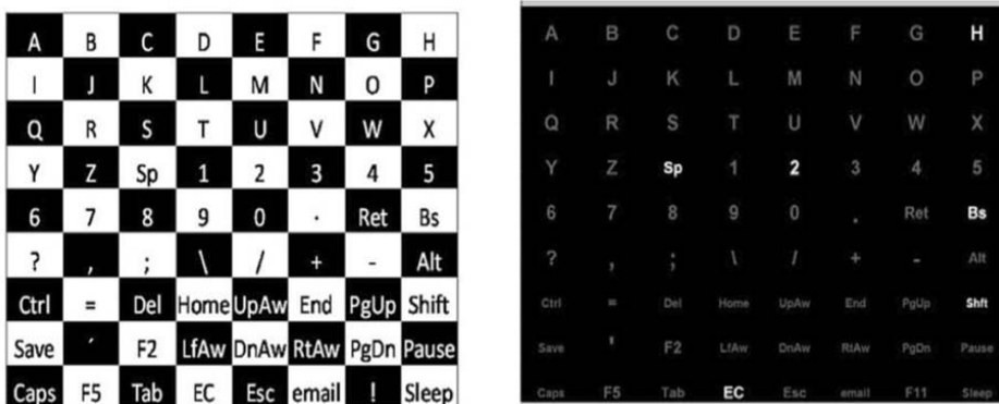
Figure 7. Checkerboard paradigm [20].
