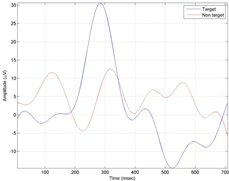
Figure 3. Temporal pattern of P300 component.
