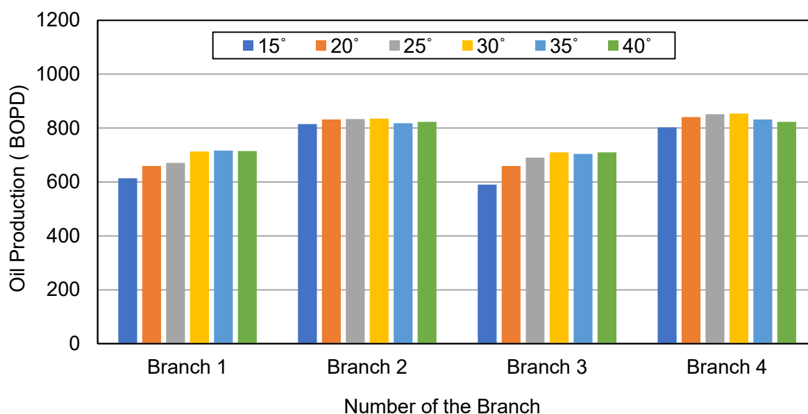
Figure 5: The effect of branche's angle on Fishbone daily production rate [39].
