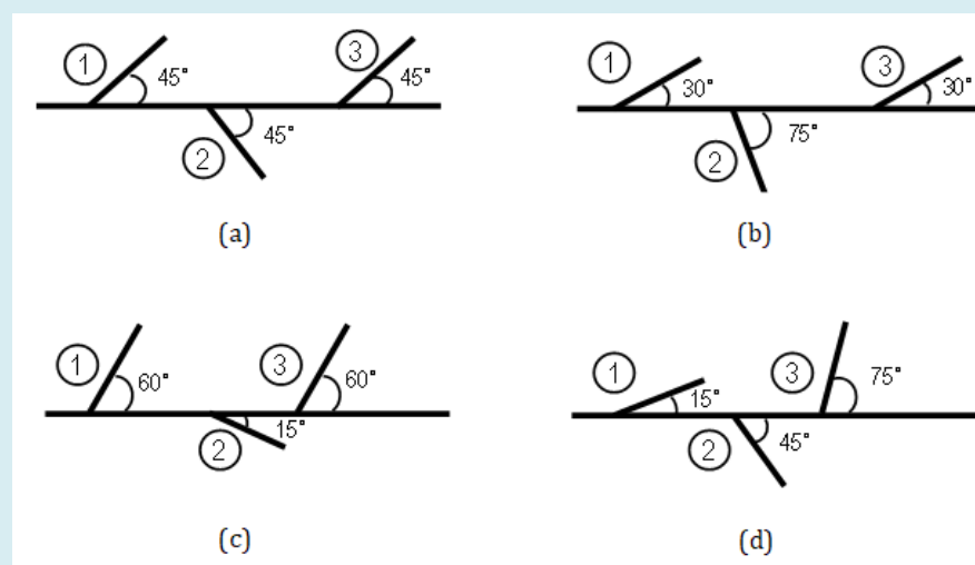
Figure 6: Schematic diagrams of four Fishbone wells geometries with different branche's angles [40].
